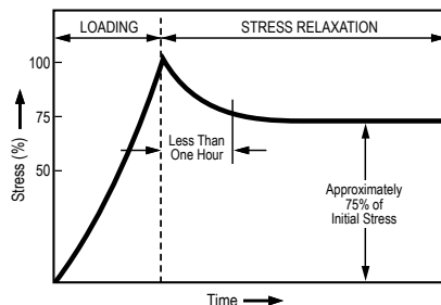
Graph 3-15. Stress Relaxation
