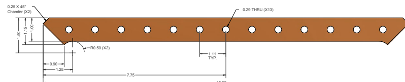
Figure 3-8. P09 Plastic Compression Stop
