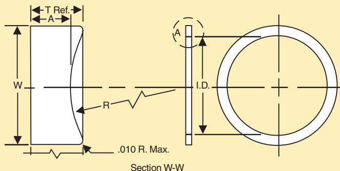
Section W-W
