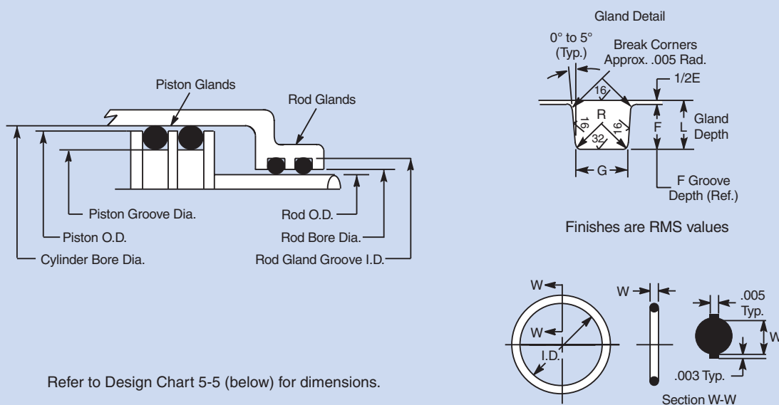
Reciprocating Vacuum Packing Glands
