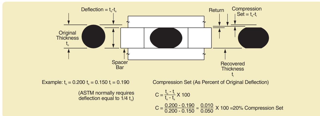
Figure 2-9: Compression Set
