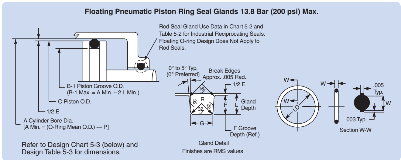
Floating Pneumatic Piston Ring Seal Glands
