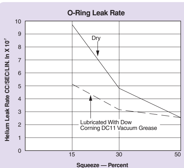
Figure 3-8: O-ring Leak Rate
