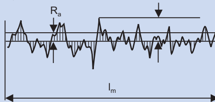
Figure 5-4: Roughness Terminology
